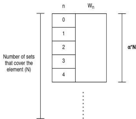
Figure 10: GRASP Algorithm
